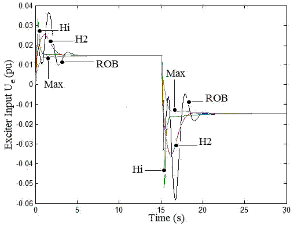
(a) Exciter Input U_e
