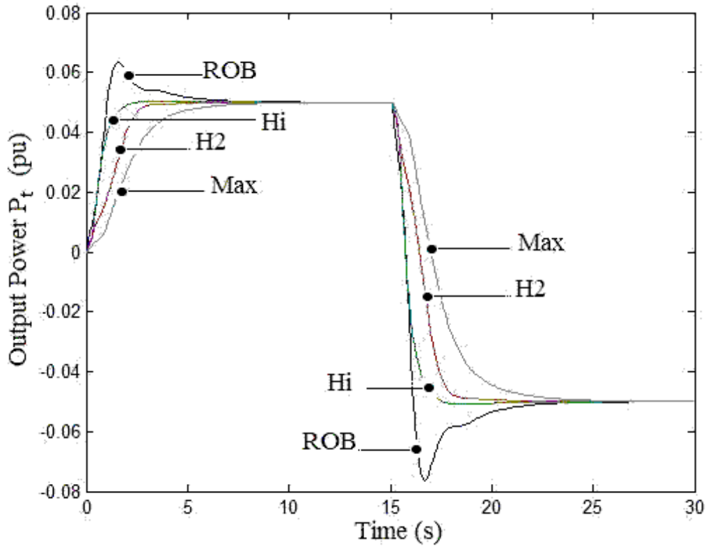
(c) Power output P_t
