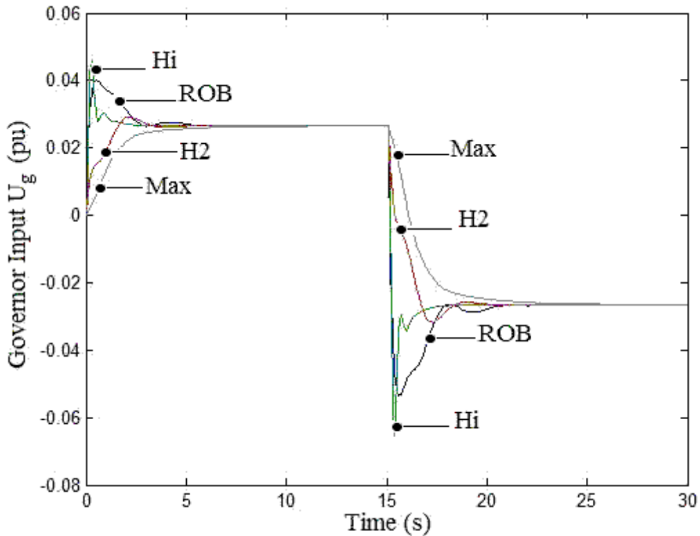
(b) Governor input U_g
