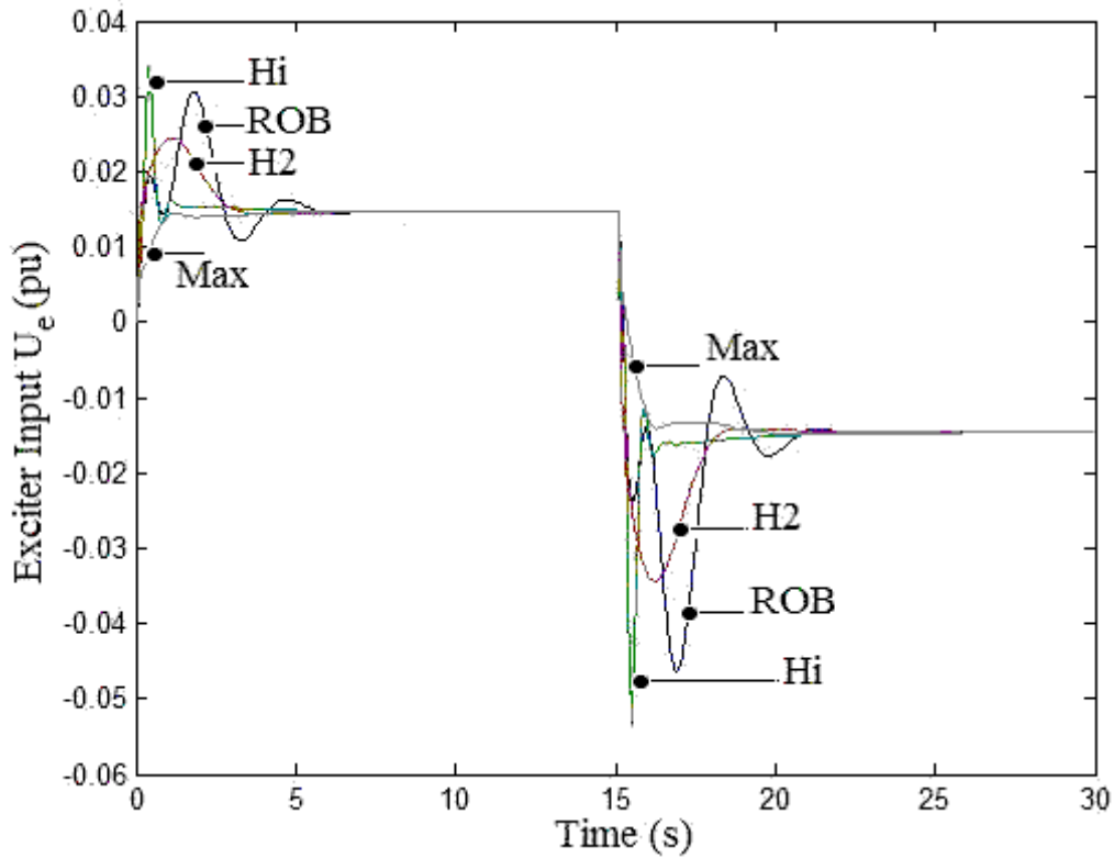
(a) Exciter Input U_e
