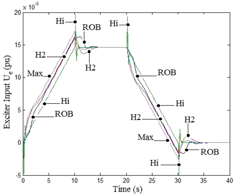
(a) Exciter Input U_e
