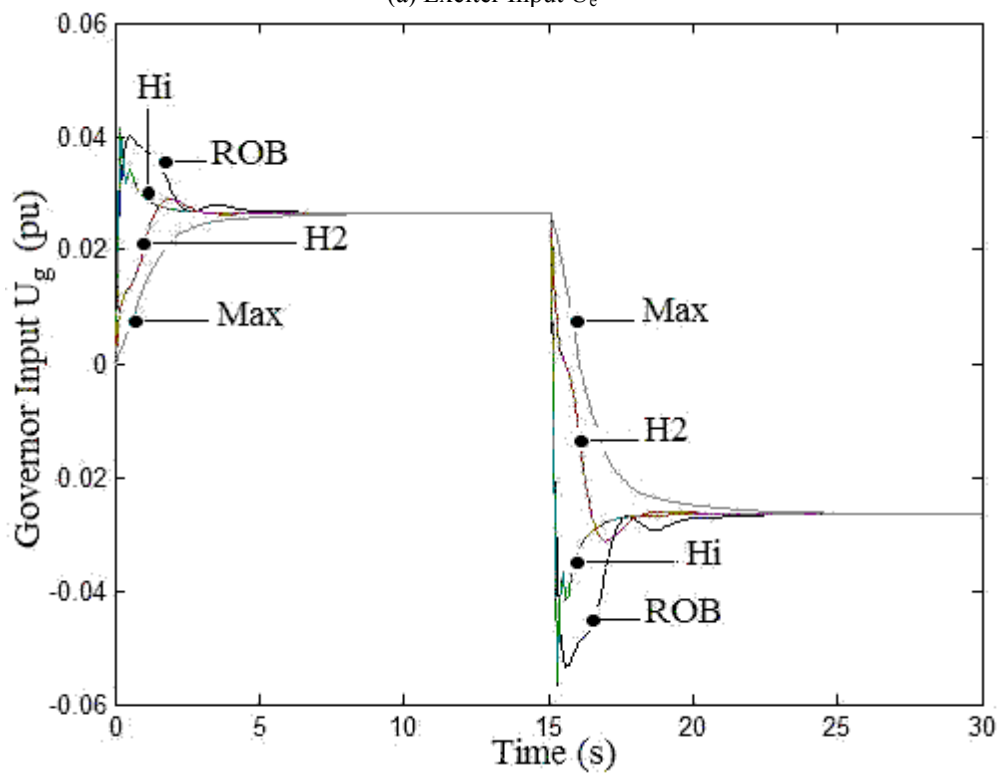
(b) Governor input U_g
