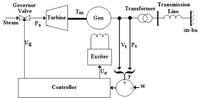
Fig. 1 Controlled sample power system
